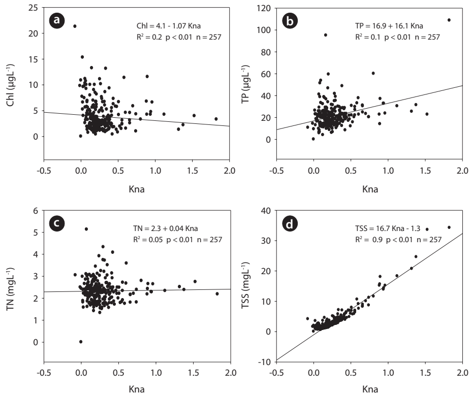
Fig. 8. Relations of chlorophyll-a (Chl), total phosphorus (TP), total nitrogen (TN), and total suspended solids (TSS) on the non-algal light attenuation (Kna) as an indicator of underwater light availability.
